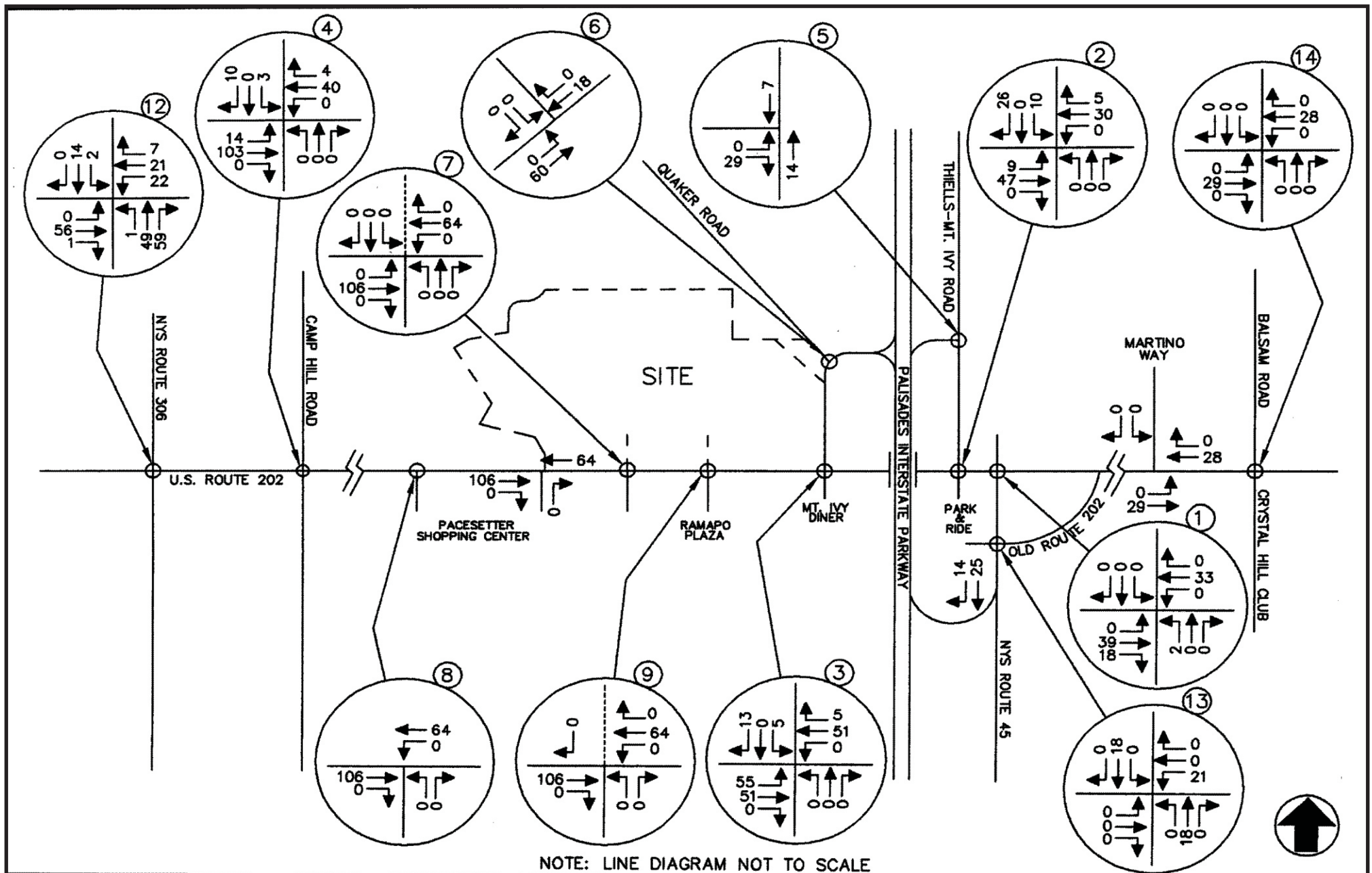
Figure 3.5-27: Other Development Traffic Volumes Weekday Peak AM Highway Hour (With Patrick Farm) Minisceongo Park Towns of Haverstraw & Ramapo, Rockland County, New York Source: John Collins Engineers, P.C. Date: October, 2008
